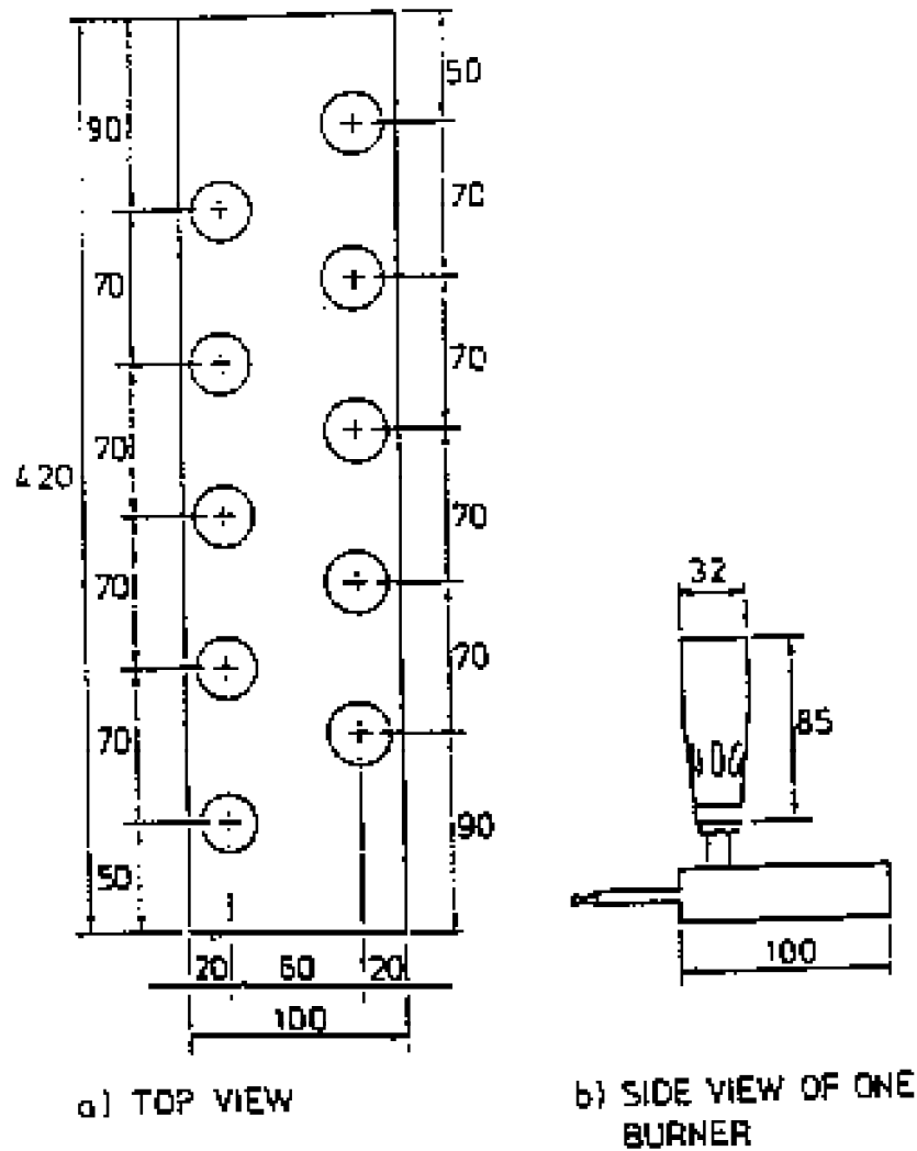
FIG. 1 FIRE ENDURANCE TEST BURNER ASSEMBLY
