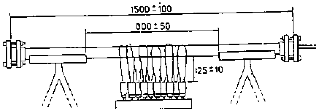
FIG. 2 FIRE ENDURANCE TEST. STAND WITH MOUNTED SAMPLE
