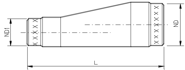
Eccentric Reducer
