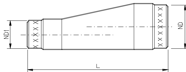
Eccentric Reducer
