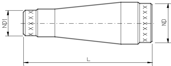
Concentric Reducer
