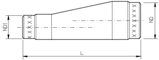
Eccentric Reducer
