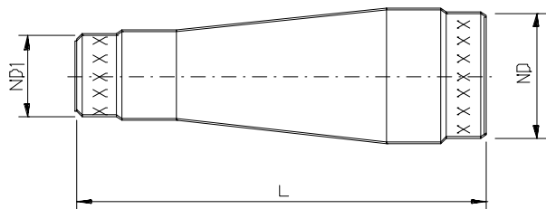
Concentric Reducer
