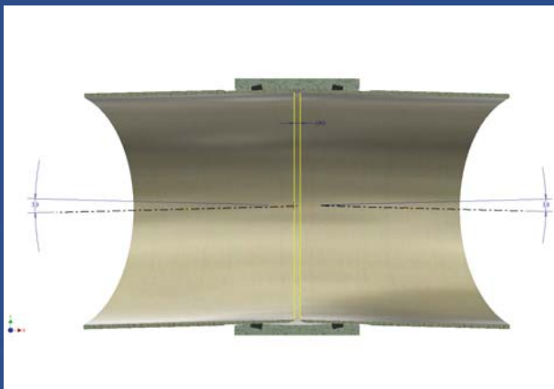
Figure 1: Double Bell and Spigot Joint with 3° Allowed Installation Angular Deflection
